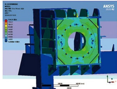
主缸安装板静力学分析 Static analysis of main bar mounting plate
