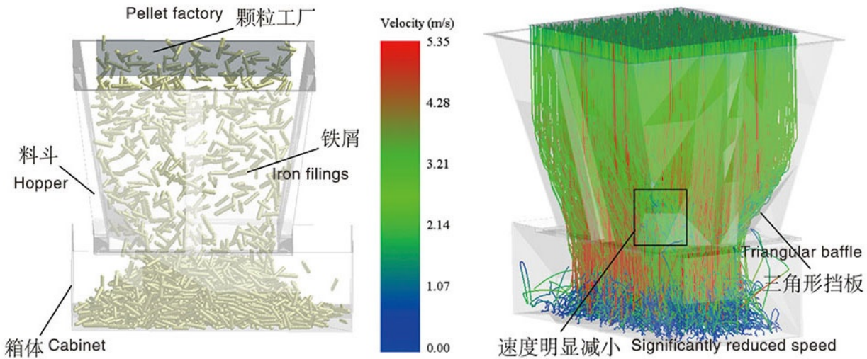
打包机静力学仿真分析结果 Static simulation analysis results of baler
