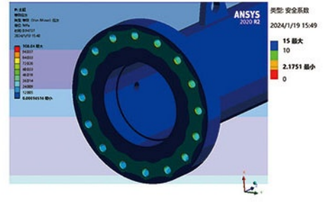
主缸静力学仿真分析 Master cylinder static simulation analysis
