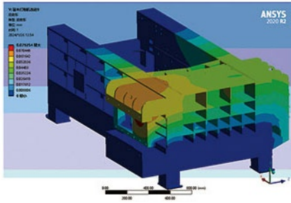
打包机静力学仿真分析结果 Static simulation analysis results of baler
